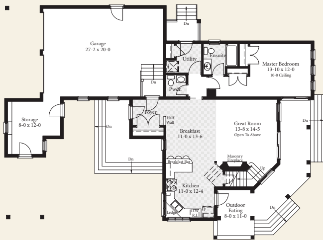
Main Floor Plan (Standard Layout)
